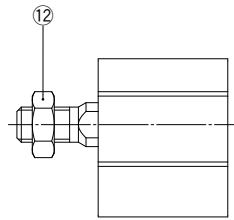
Rod end male threaded
