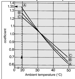
Correction Factor by Ambient Temperature
