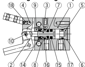
Double acting/With fingers open
