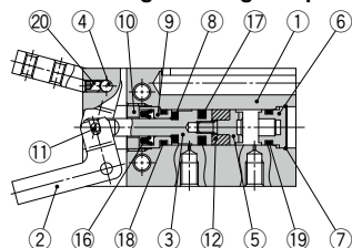
Double acting/With fingers open
