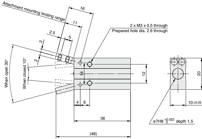
Auto switch mounting groove dimensions
