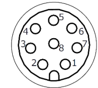
M8 connector pin layout
